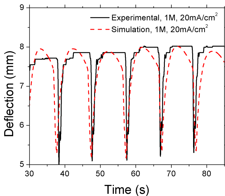
Figure 4.4: Oscillating tip displacement. Experimental [19] data and simulation data for 1 M HCHO solution, applied current density of 20 mA/cm^2 .
