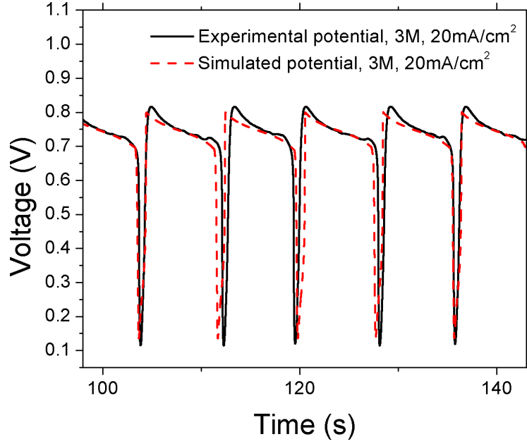
Figure 4.3: Potential oscillations. Measured data [19] and simulated data for 3 M HCHO solution. The potential oscillations were measured between the cathode and anode of the IPMC strip during the experiment. The applied current was maintained at constant value of 20 \text{ mA/cm}^2 .
