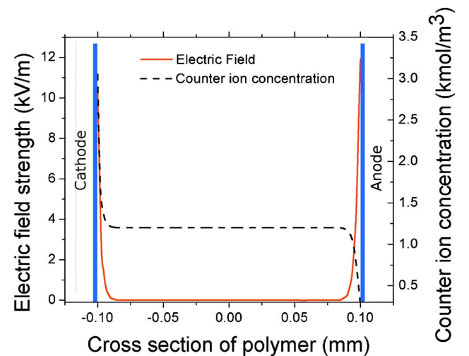
FIG. 2. (Color online) The concentration of counterions and the electric field strength inside the polymer according to simulations for a potential of 2 V.
