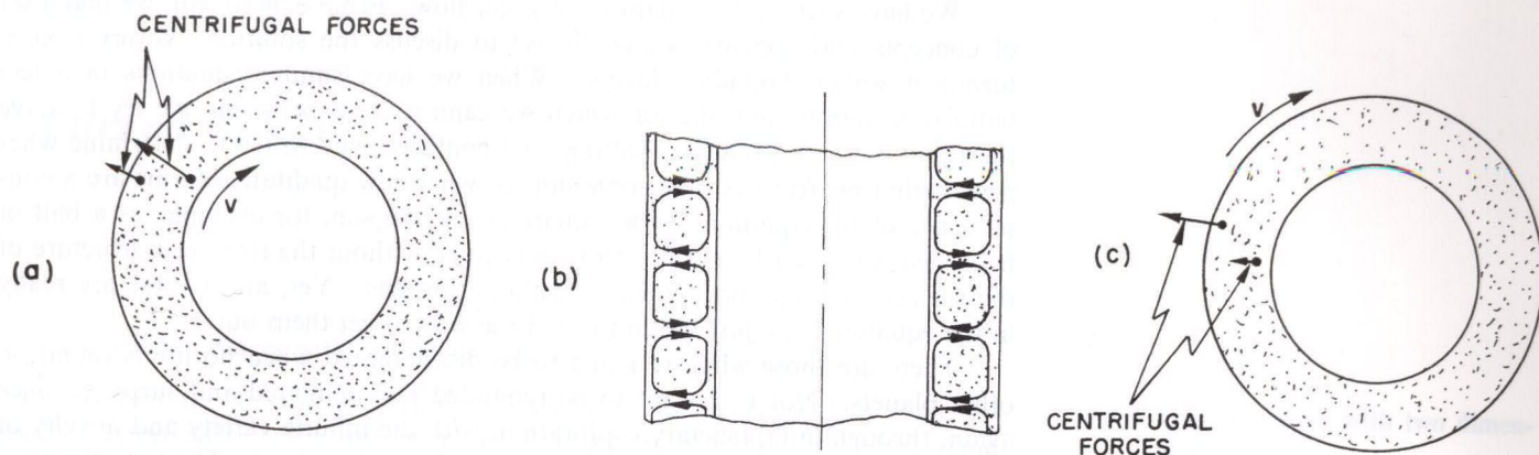
Fig. 41-9. Why the flow breaks up into bands.
