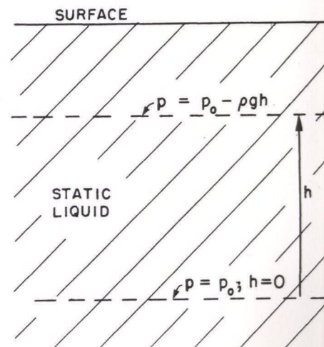
Fig. 40-2. The pressure in a static liquid.
