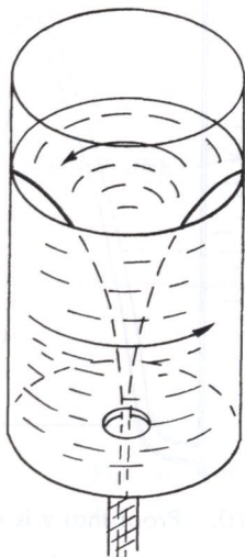
Fig. 40-12. Water with circulation draining from a tank.
