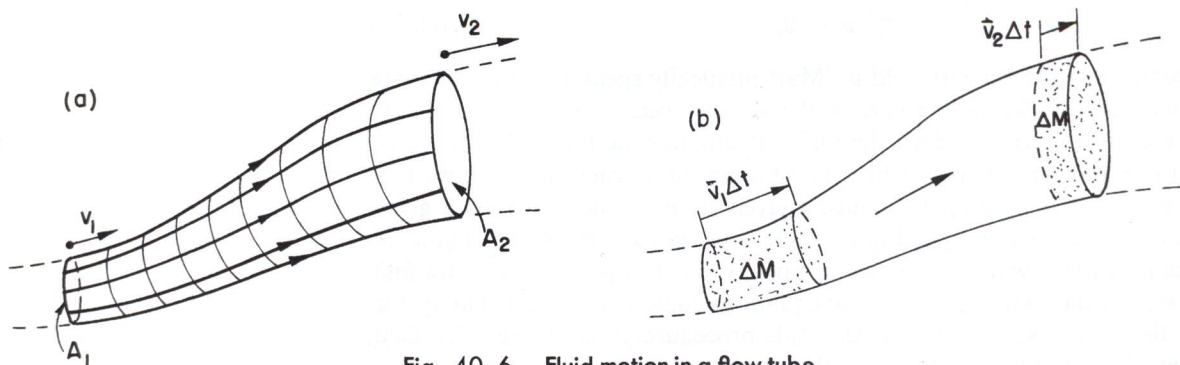
Fig. 40-6. Fluid motion in a flow tube.
