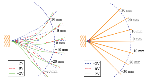
Fig.4. Static equilibrium states of a long IPMC manipulator (left) and a short IPMC manipulator with a rigid elongation (right)
